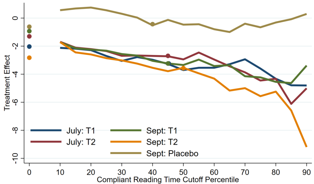
Figure D3: Treatment Effects on Compliant and Uninformed Respondents by Reading Time Percentile
