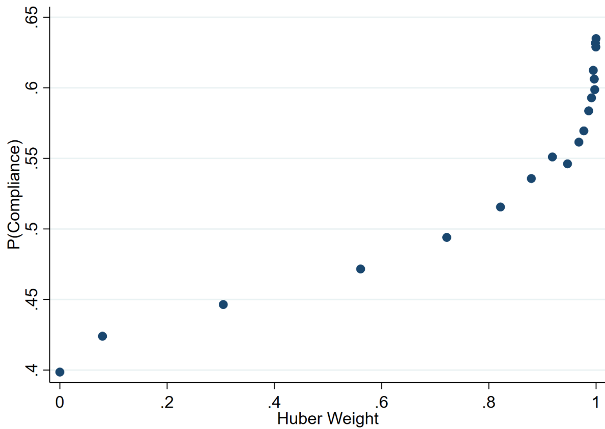
Figure D2: Compliance Probabilities vs. Huber Weights
